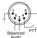
C 0379 5 Pin XLR Wiring Diagram
