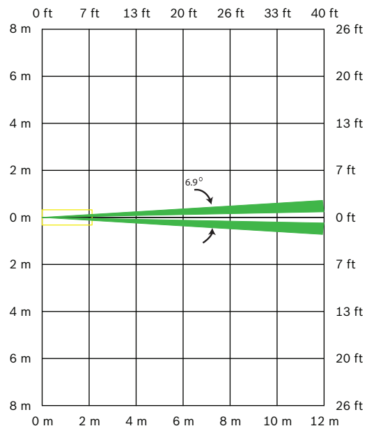
Top View Broad: 12 m x 1.5 m (40 ft x 5 ft)
