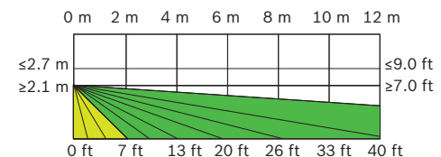
Side View Broad: 12 m x 12 m (40 ft x 40 ft)
