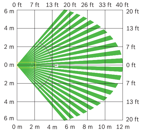
Top View Broad: 12 m x 12 m (40 ft x 40 ft)
