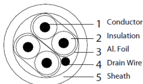
Cable Construction Relative Parts
