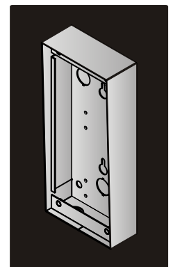
stainless steel guard enclosure model: ENCGRDSSV height: 225.0mm width: 100.0mm depth: 45.0mm
