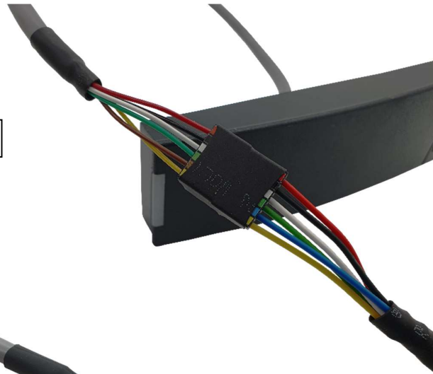
FAST-R6J – Weigand Reader Joiner
