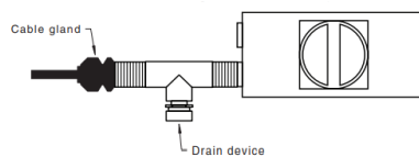
Example of a device to drain liquid from a conduit system (side entry/exit)
