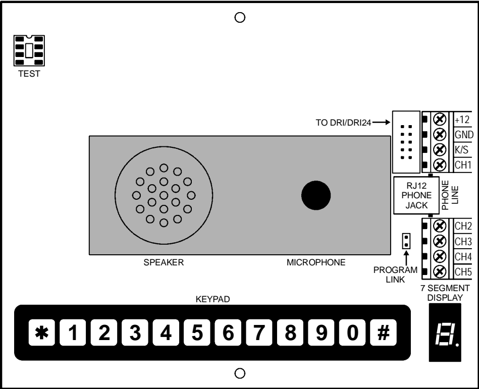
Figure 1: The DT6I with its outer cover removed.
