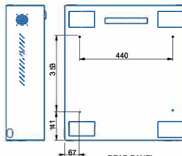
REAR PANEL
