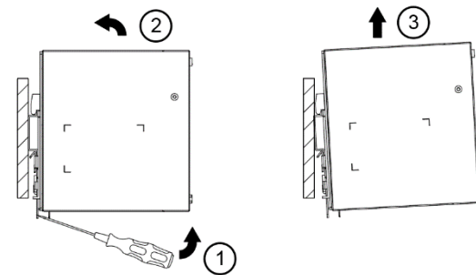
Fig. 3.2 Dismounting
