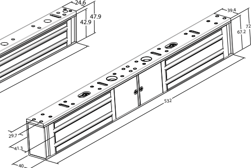
Z8 Electromagnetic Lock
