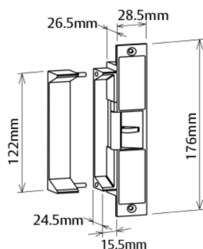
ES9000 with 25mm Extension Lip
