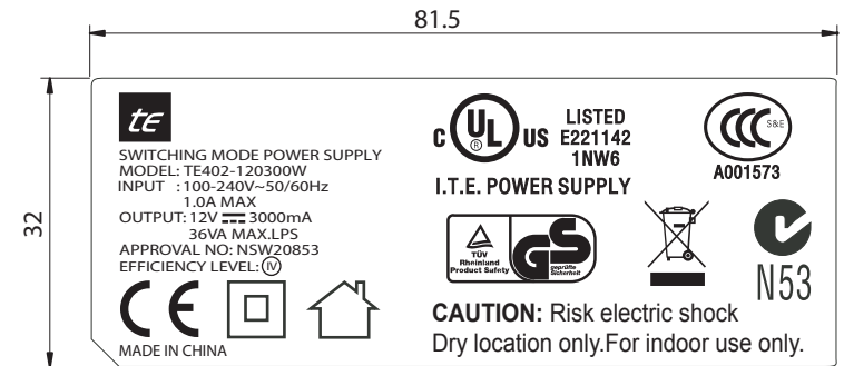
LABEL ARTWORK Black words on silver base label
