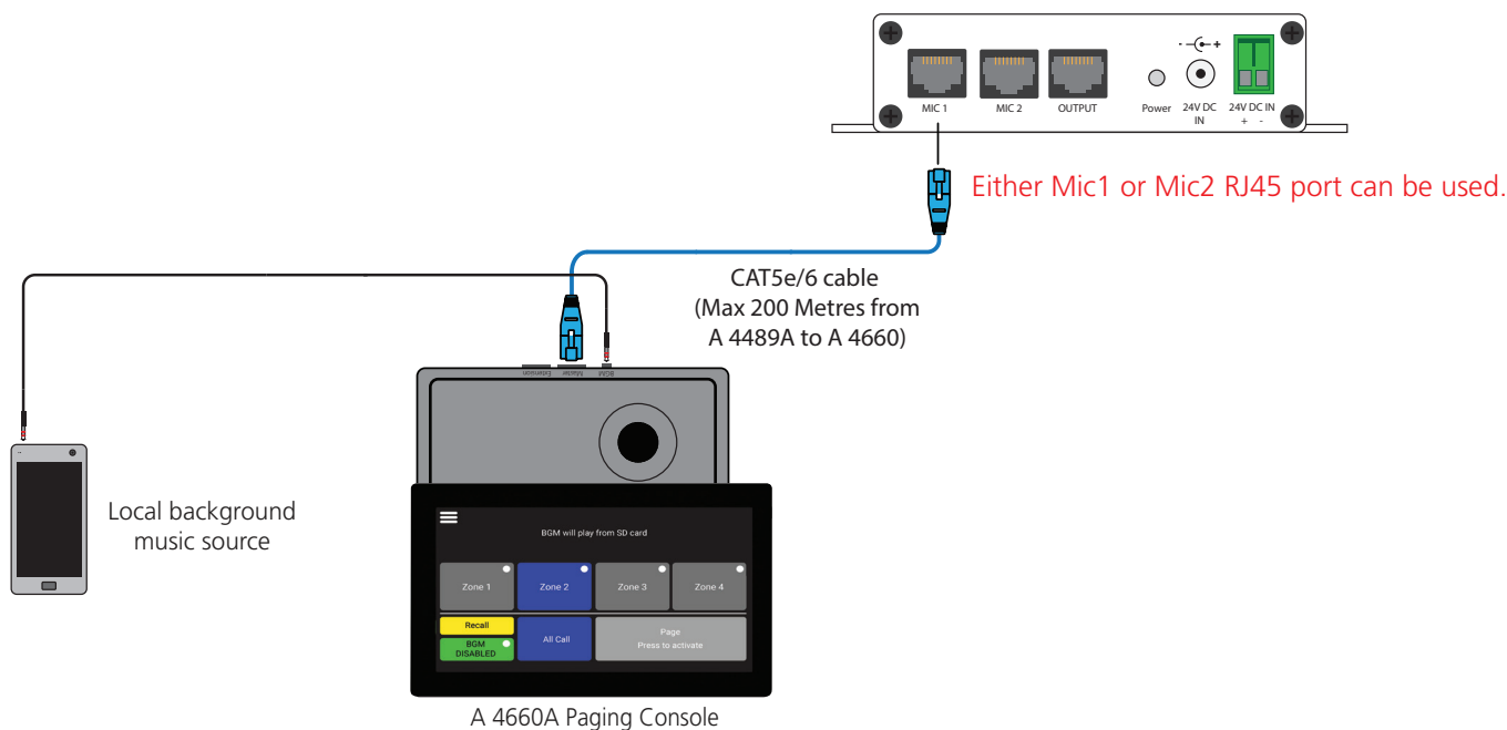
Fig 15 - Local BGM input via Redback A 4944 solutions transmitter
