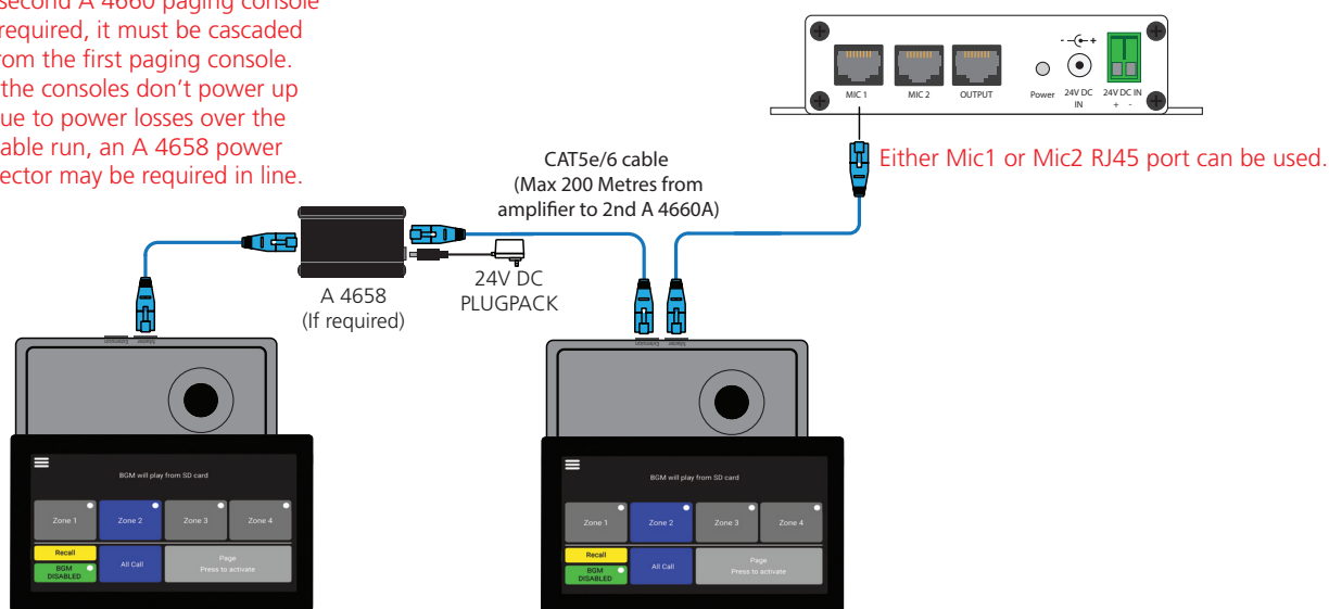
Fig 8 Cascading A 4660A paging consoles.
