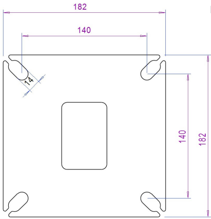
BASEPLATE FOR SQ &SEQ
