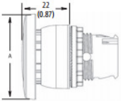
Mushroom Operators (40 mm and 60 mm)
