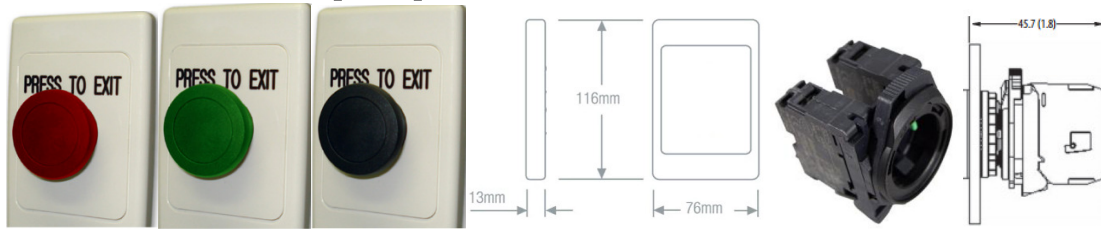
Mushroom Operators (40 mm and 60 mm)
