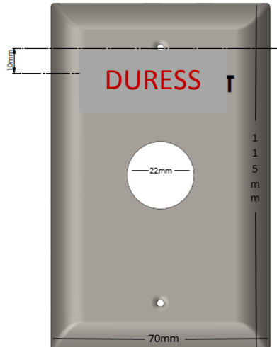
40 mm Key Release Mushroom Cat. No. 800FP-MK44
