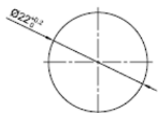
PANEL CUTOUT MAX.PANEL THICKNESS 8 mm
