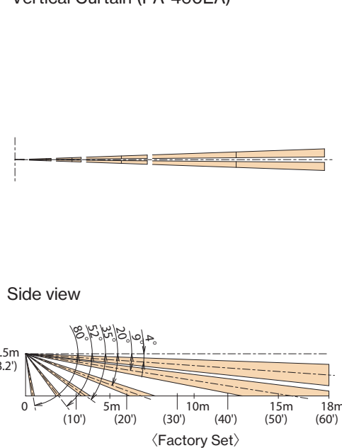
Vertical Curtain (PA-460EA)
