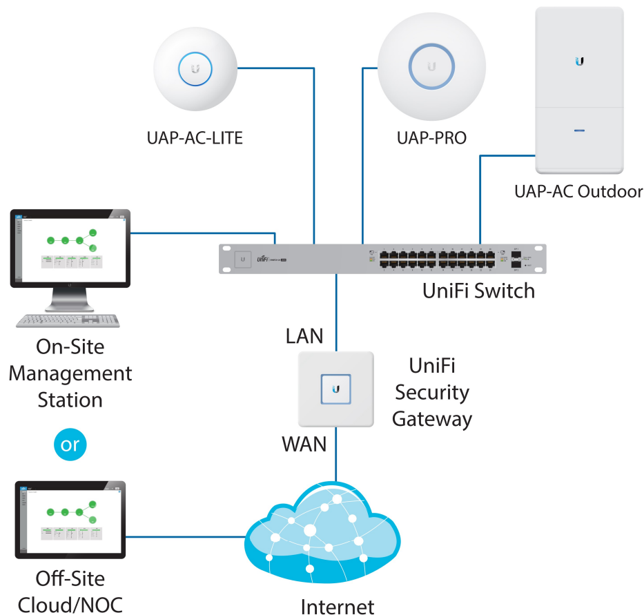
Sample Network Diagram
